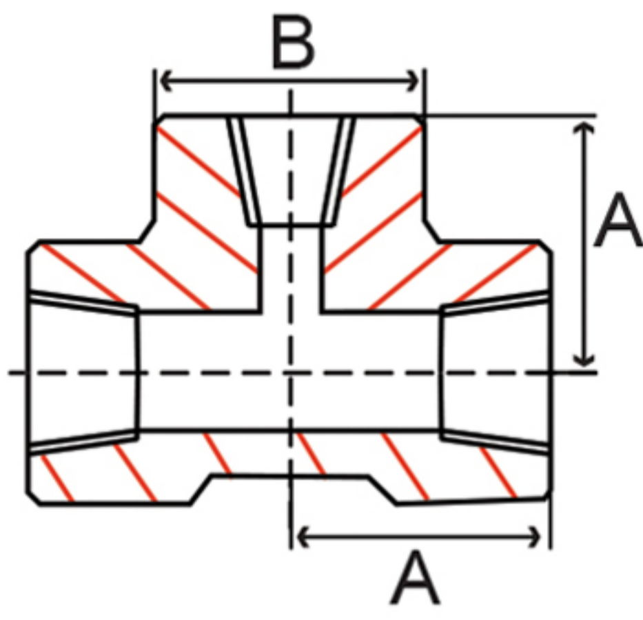
Fig. 42RT3 – Reducing Tee
